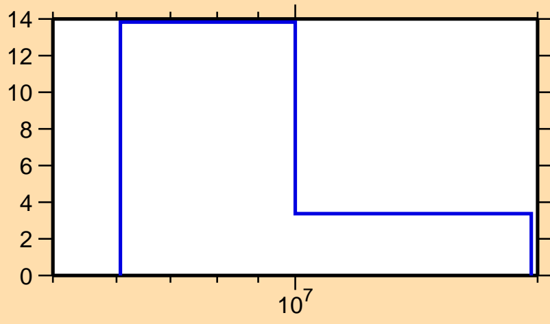
\Delta\sigma/\sigma vs. E for ^{163}\text{Er}(n,2n)
