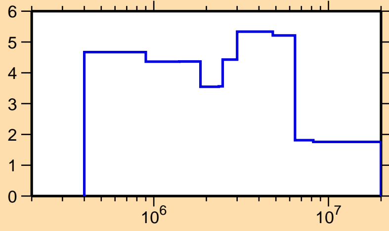
\Delta\sigma/\sigma vs. E for ^{163}\text{Er}(n, el.)
