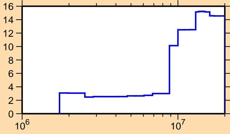
\Delta\sigma/\sigma vs. E for ^{164}\text{Er}(n,n\text{cont.})
