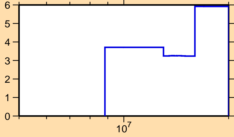
\Delta\sigma/\sigma vs. E for ^{164}\text{Er}(n,2n)
