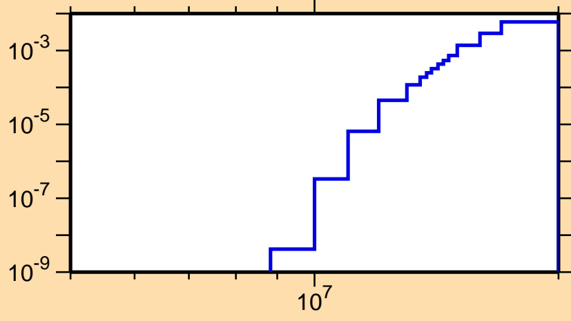
\sigma vs. E for ^{164}\text{Er}(n,np)
