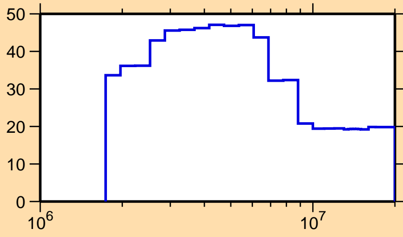
\Delta\sigma/\sigma vs. E for ^{164}\text{Er}(n,\gamma)
