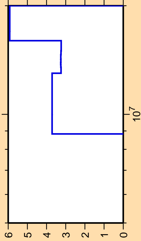
\Delta\sigma/\sigma vs. E for ^{164}\text{Er}(n,2n)
