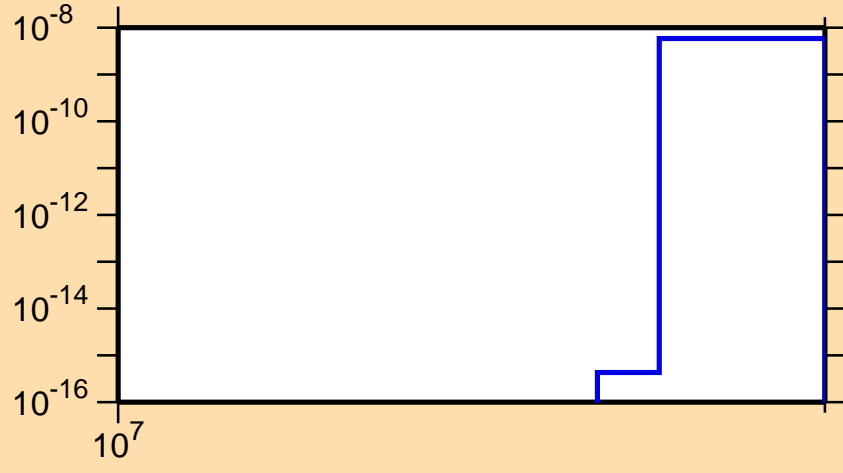
\sigma vs. E for ^{164}\text{Er}(n,2np)
