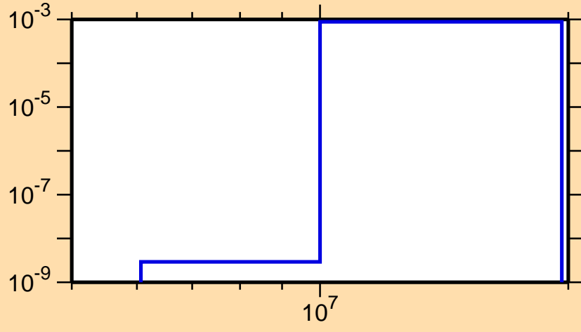
\sigma vs. E for ^{164}\text{Er}(n,d)
