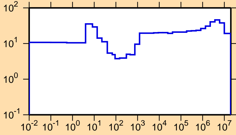
\Delta\sigma/\sigma vs. E for ^{164}\text{Er}(n,\gamma)
