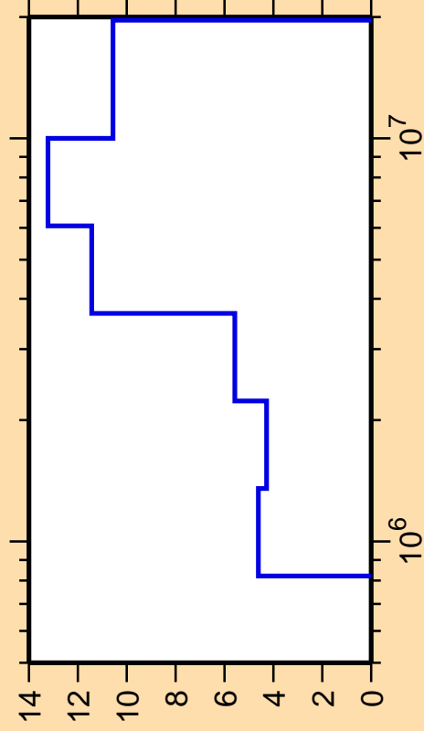
\Delta\sigma/\sigma vs. E for ^{164}\text{Er}(n,n_4)
