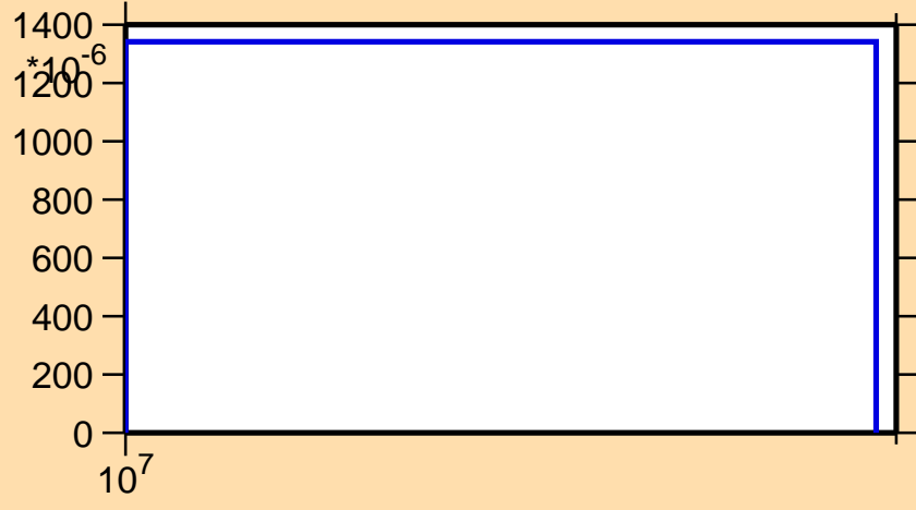
\sigma vs. E for ^{164}\text{Er}(n,3n)
