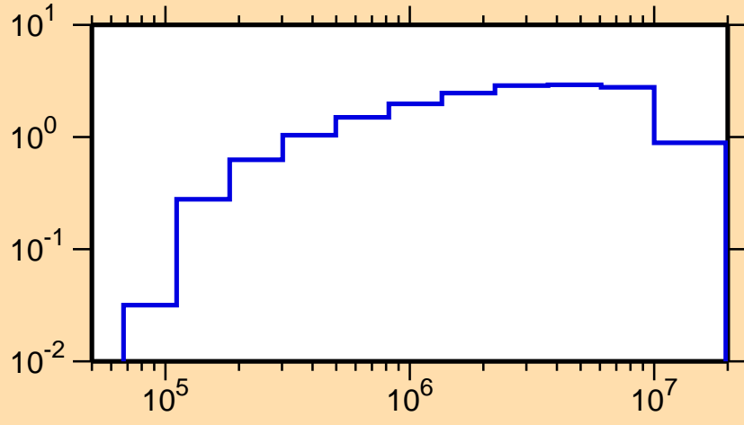
\sigma vs. E for ^{164}\text{Er}(n,\text{inel.})
