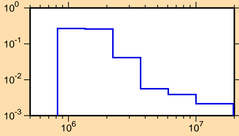
\sigma vs. E for ^{164}\text{Er}(n,n_4)
