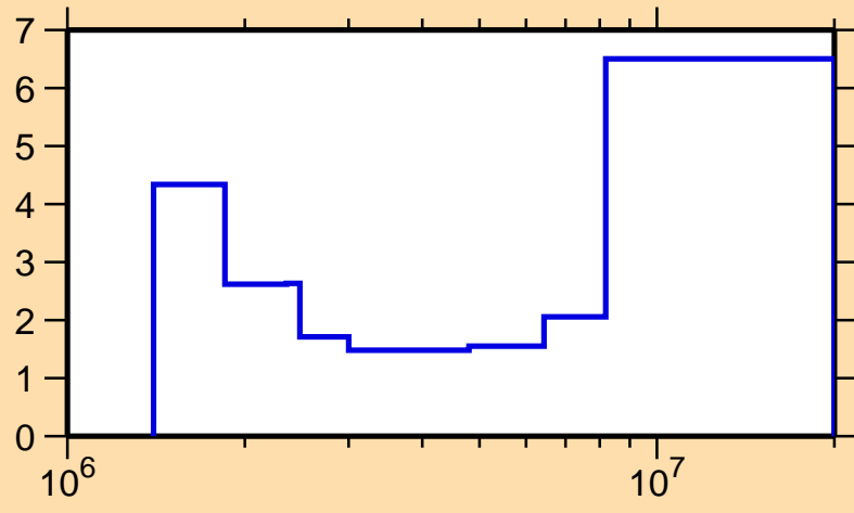
\Delta\sigma/\sigma vs. E for ^{164}\text{Er}(n,\text{inel.})
