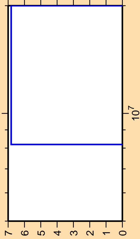
\Delta\sigma/\sigma vs. E for ^{164}\text{Er}(n,n_1)
