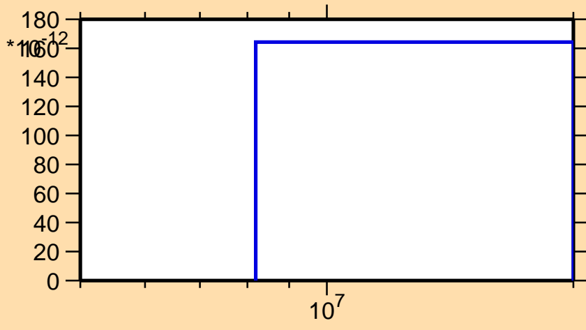
\sigma vs. E for ^{164}\text{Er}(n,\text{He3})
