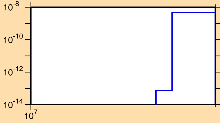
\sigma vs. E for ^{165}\text{Er}(n,nt)
