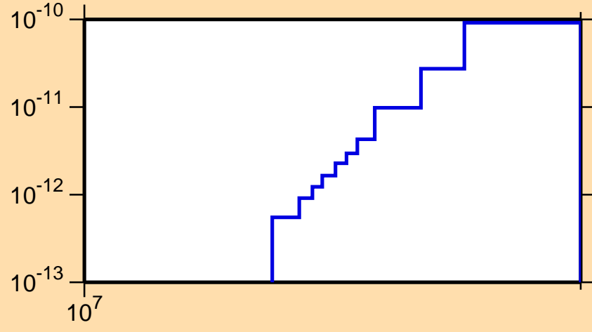
\sigma vs. E for ^{165}\text{Er}(n,p\alpha)
