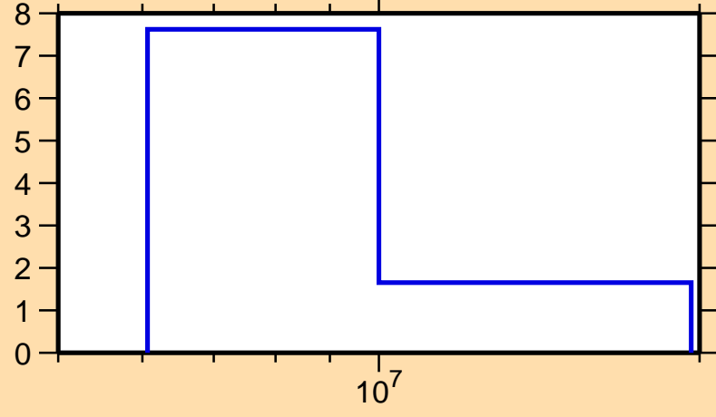
\Delta\sigma/\sigma vs. E for ^{165}\text{Er}(n,2n)
