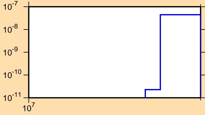
\sigma vs. E for ^{166}\text{Er}(n,\text{nd})
