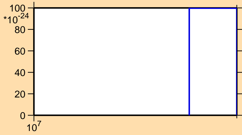
\sigma vs. E for ^{166}\text{Er} (mt 11)
