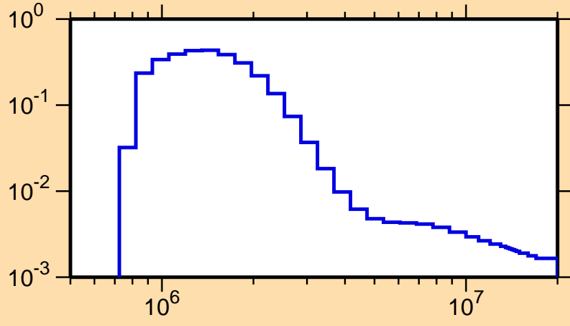
\sigma vs. E for ^{166}\text{Er}(n,n_4)
