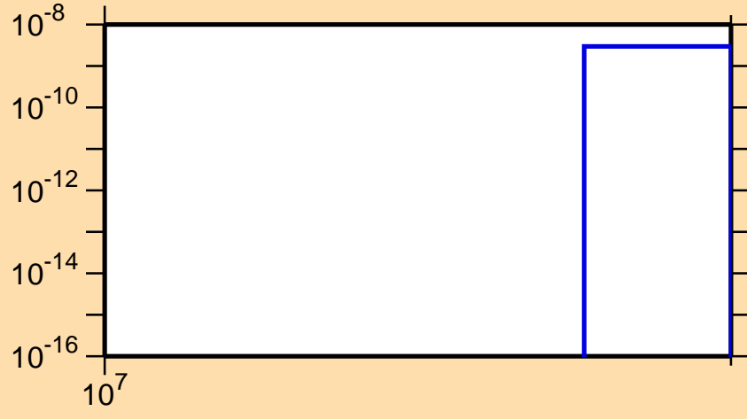
\sigma vs. E for ^{166}\text{Er}(n,2np)
