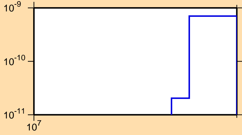
\sigma vs. E for ^{166}\text{Er}(n,\text{He3})
