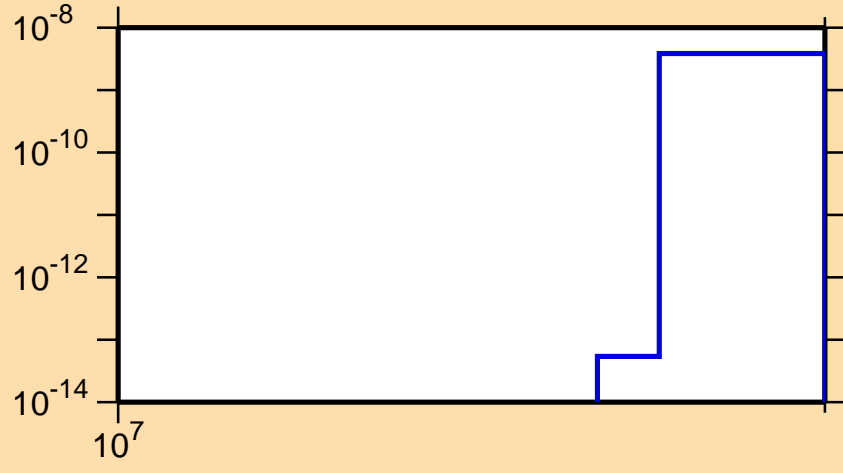
\sigma vs. E for ^{166}\text{Er}(n,nt)
