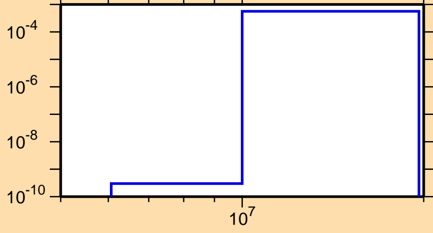
\sigma vs. E for ^{166}\text{Er}(n,d)
