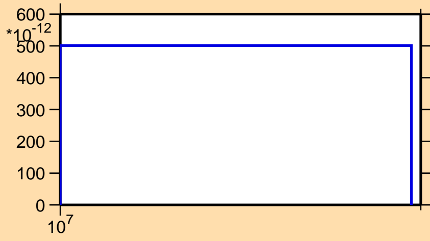
\sigma vs. E for ^{166}\text{Er}(n,2n\alpha)
