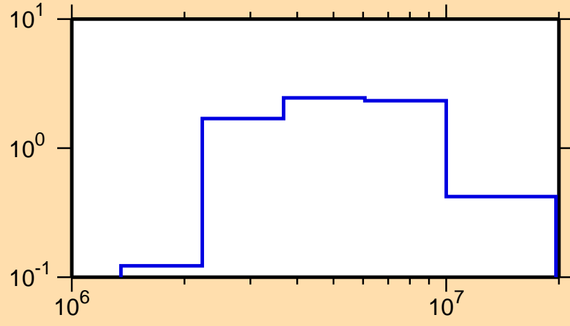
\sigma vs. E for ^{166}\text{Er}(n,n\text{cont.})
