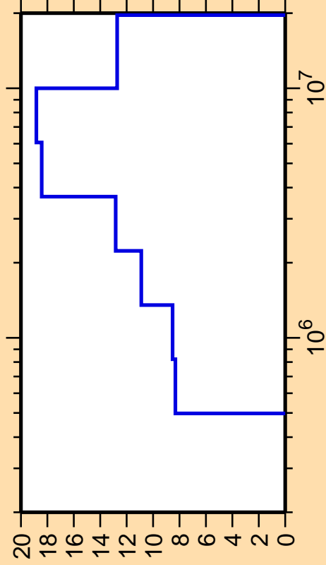
\Delta\sigma/\sigma vs. E for ^{166}\text{Er}(n,n_3)
