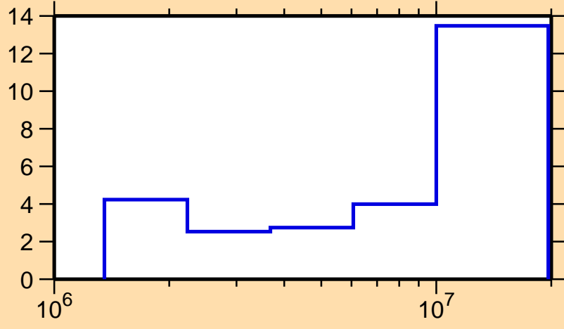
\Delta\sigma/\sigma vs. E for ^{166}\text{Er}(n,n\text{cont.})
