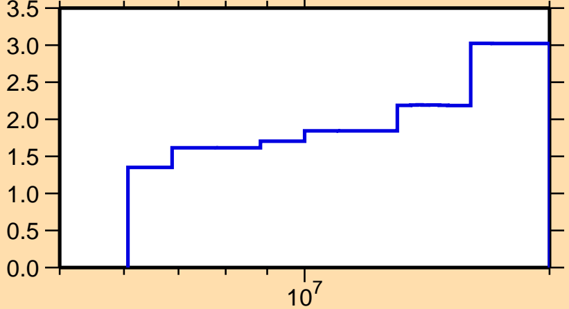
\Delta\sigma/\sigma vs. E for ^{167}\text{Er}(n,\text{el.})
