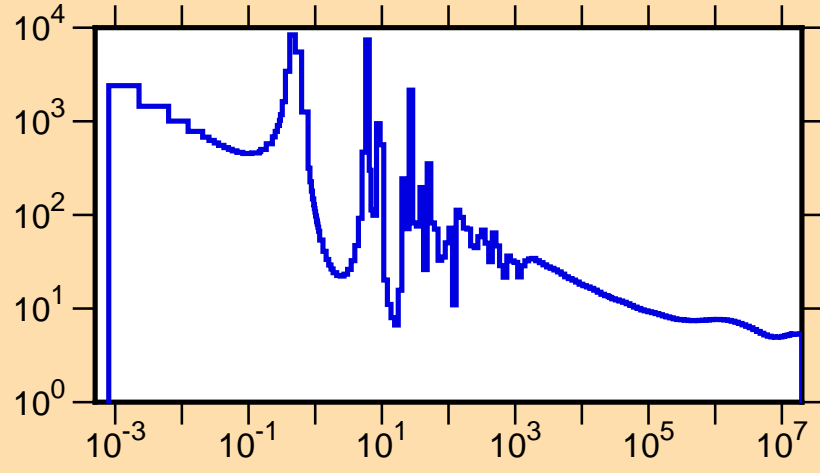
\sigma vs. E for ^{167}\text{Er}(n,\text{tot.})
