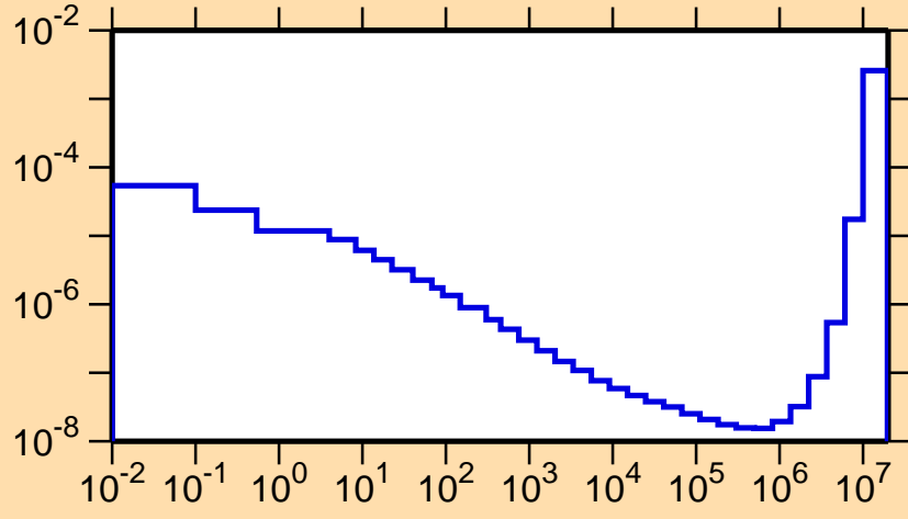
\sigma vs. E for ^{167}\text{Er}(n,\alpha)
