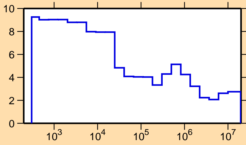
\Delta\sigma/\sigma vs. E for ^{167}\text{Er}(n,\text{nonel.})
