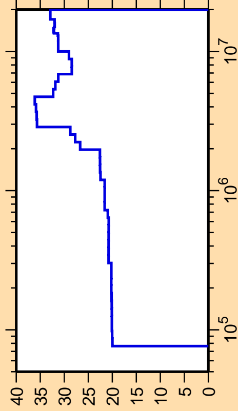
\Delta\sigma/\sigma vs. E for ^{168}\text{Er}(n,\gamma)
