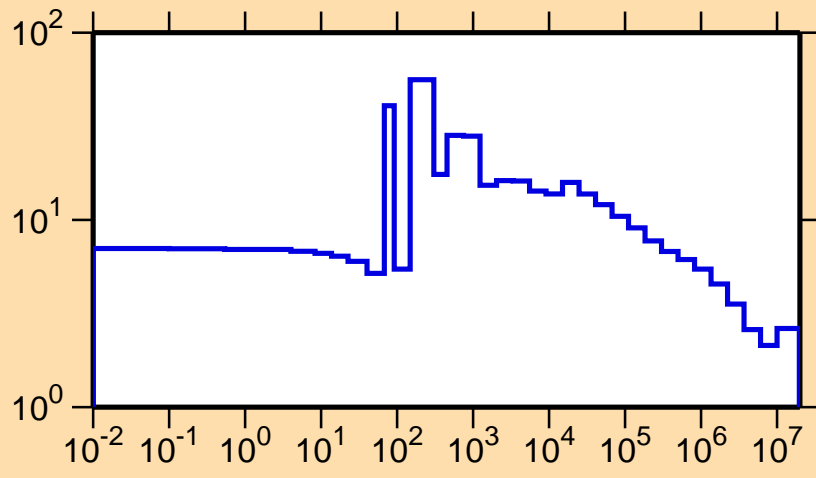
\sigma vs. E for ^{168}\text{Er}(n,\text{el.})
