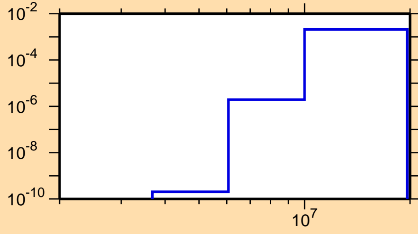
\sigma vs. E for ^{168}\text{Er}(n,p)
