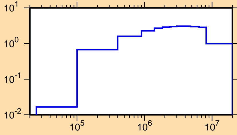
\sigma vs. E for ^{168}\text{Er}(n,\text{inel.})
