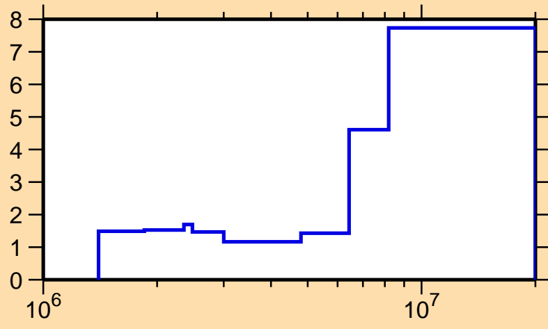
\Delta\sigma/\sigma vs. E for ^{168}\text{Er}(n,\text{inel.})
