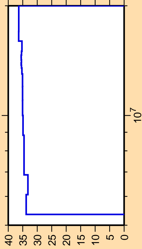
\Delta\sigma/\sigma vs. E for ^{169}\text{Er}(n,\gamma)
