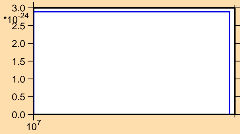
\sigma vs. E for ^{169}\text{Er} (mt 11)
