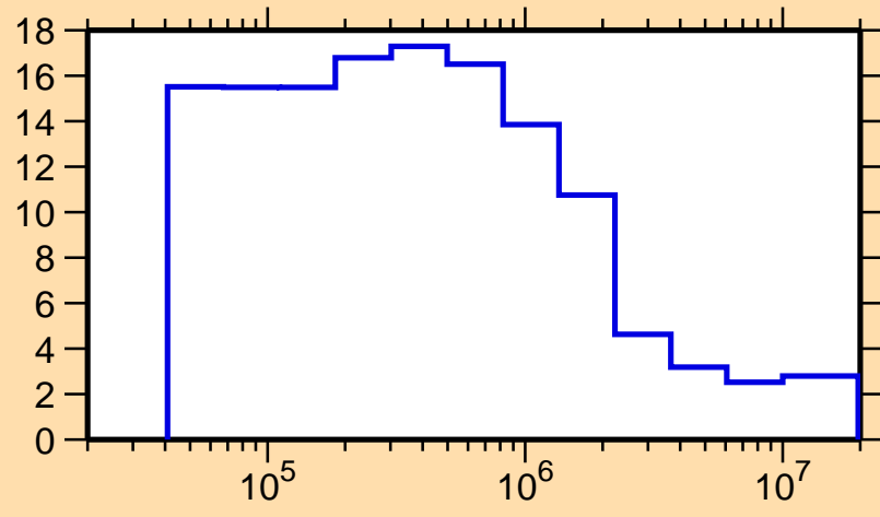
\Delta\sigma/\sigma vs. E for ^{169}\text{Er}(n,\text{nonel.})
