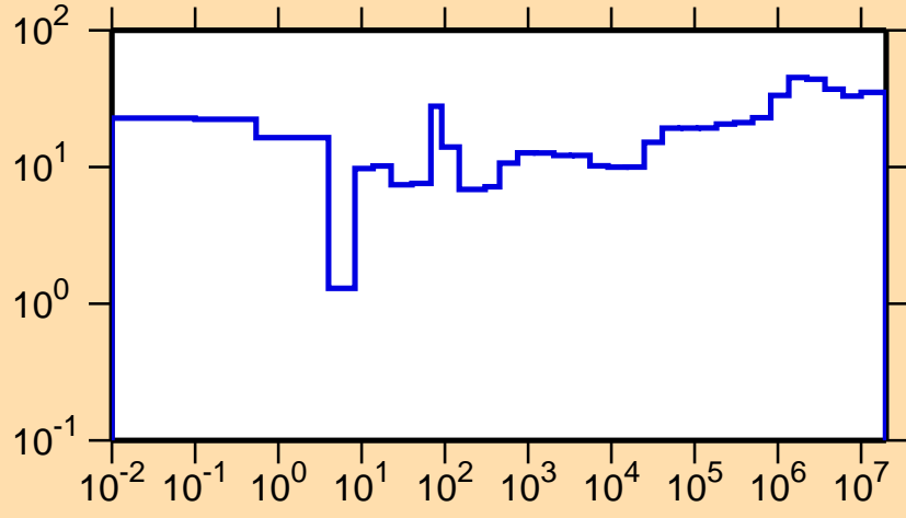
\Delta\sigma/\sigma vs. E for ^{169}\text{Er}(n,\gamma)
