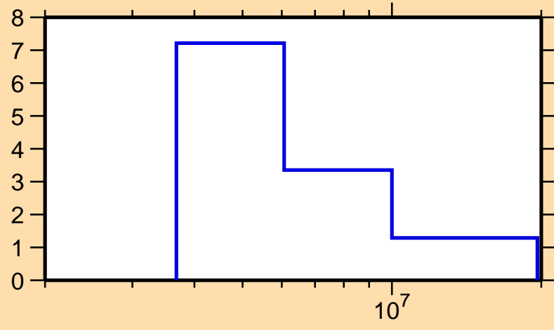
\Delta\sigma/\sigma vs. E for ^{169}\text{Er}(n,\text{el.})
