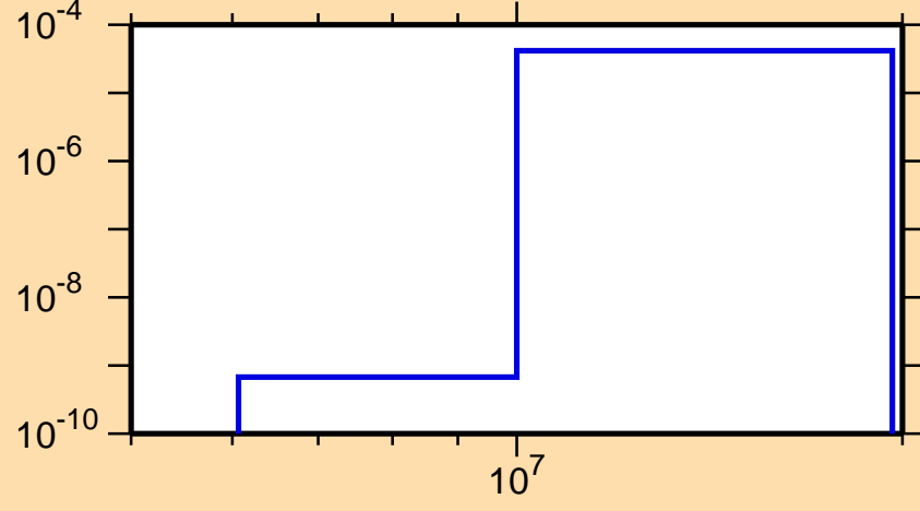
\sigma vs. E for ^{169}\text{Er}(n,n\alpha)
