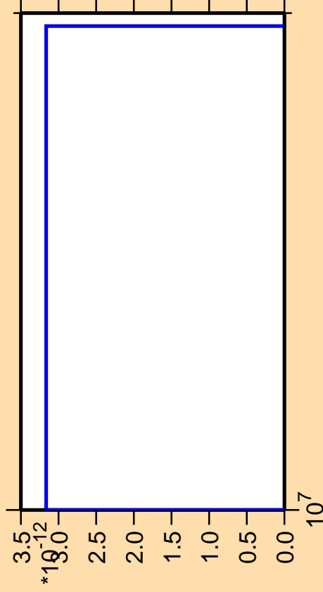
\Delta\sigma/\sigma vs. E for ^{169}\text{Er} (mt 11)
