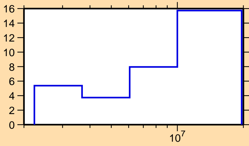
\Delta\sigma/\sigma vs. E for ^{169}\text{Er}(n,n\text{cont.})
