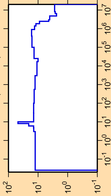
\Delta\sigma/\sigma vs. E for ^{169}\text{Er}(n,\text{nonel.})
