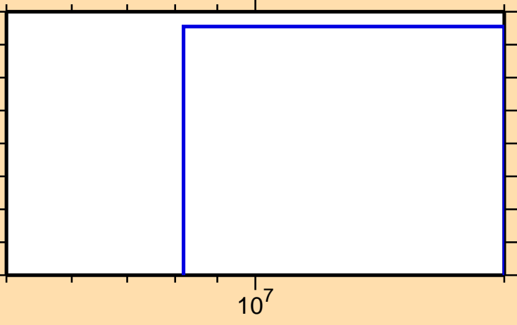
\sigma vs. E for ^{169}\text{Er}(n,np)
