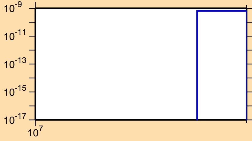
\sigma vs. E for ^{170}\text{Er}(n,2np)
