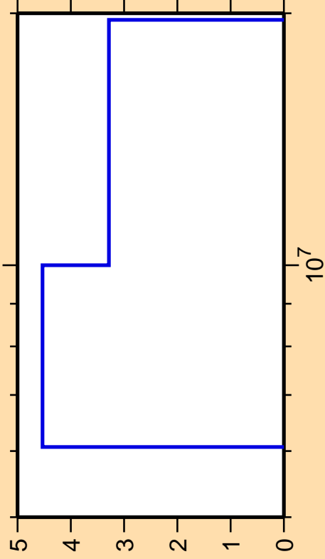
\Delta\sigma/\sigma vs. E for ^{170}\text{Er}(n,2n)
