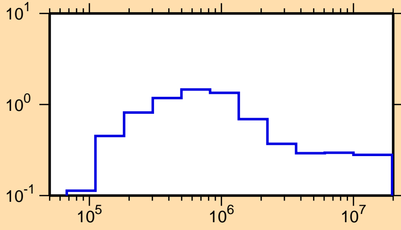
\sigma vs. E for ^{170}\text{Er}(n,n_1)
