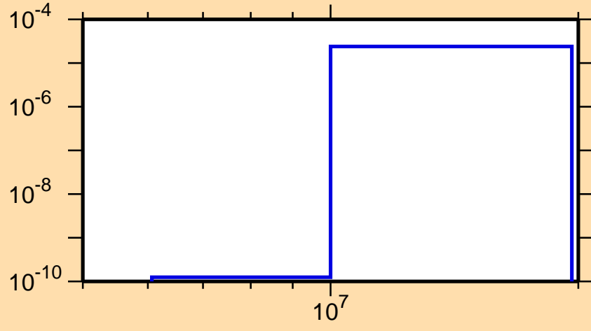
\sigma vs. E for ^{170}\text{Er}(n,n\alpha)
