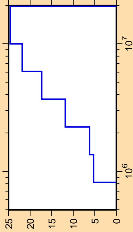
\Delta\sigma/\sigma vs. E for ^{170}\text{Er}(n,n_4)
