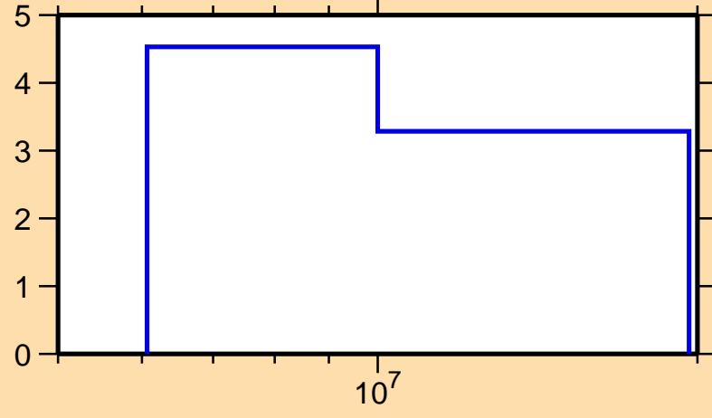
\Delta\sigma/\sigma vs. E for ^{170}\text{Er}(n,2n)
