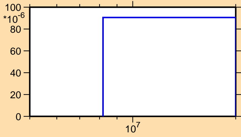
\sigma vs. E for ^{171}\text{Er}(n,d)
