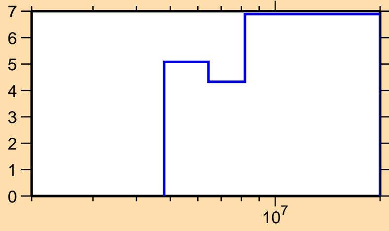
\Delta\sigma/\sigma vs. E for ^{171}\text{Er}(n,2n)
