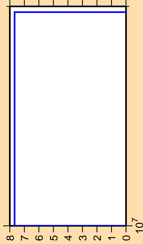
\Delta\sigma/\sigma vs. E for ^{172}\text{Er}(n,3n)
