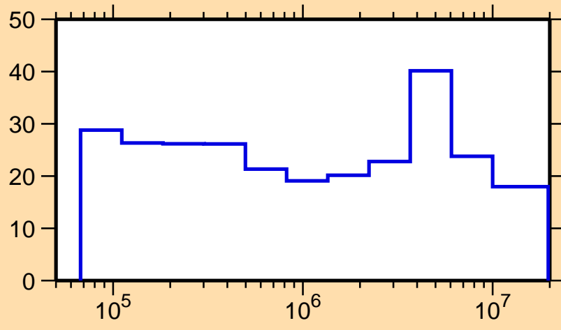
\Delta\sigma/\sigma vs. E for ^{172}\text{Er}(n,n_1)
