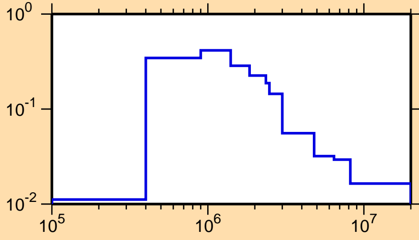
\sigma vs. E for ^{172}\text{Er}(n,n_2)
