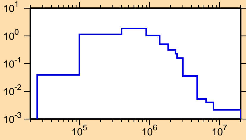
\sigma vs. E for ^{172}\text{Er}(n,n_1)
