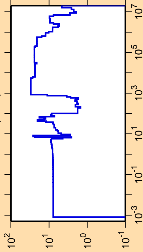
\Delta\sigma/\sigma vs. E for ^{173}\text{Er}(n,\text{el.})
