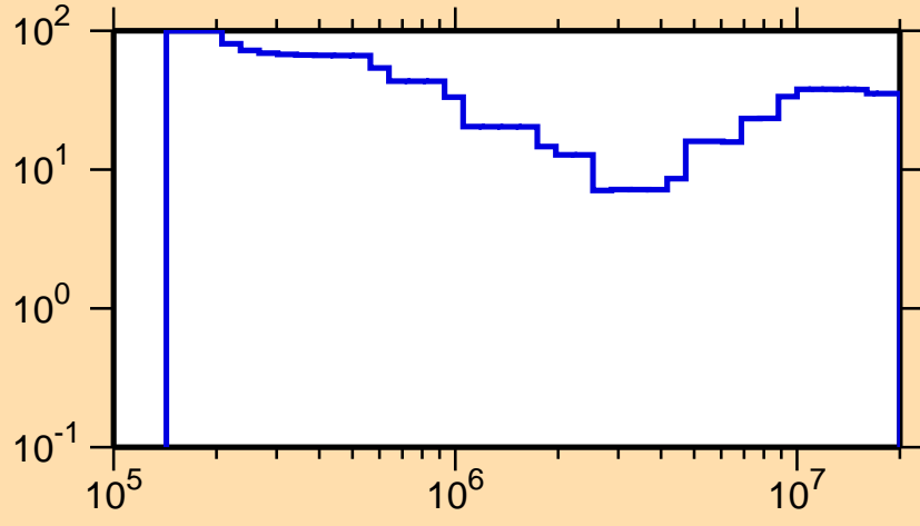
\Delta\sigma/\sigma vs. E for ^{173}\text{Er}(n,n\text{cont.})
