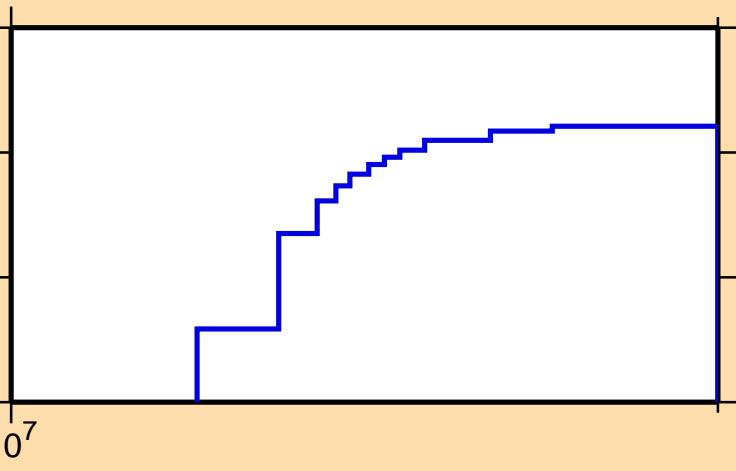
\sigma vs. E for ^{173}\text{Er}(n,3n)
