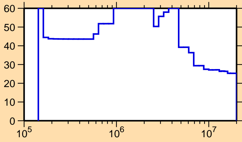
\Delta\sigma/\sigma vs. E for ^{173}\text{Er}(n,n_1)
