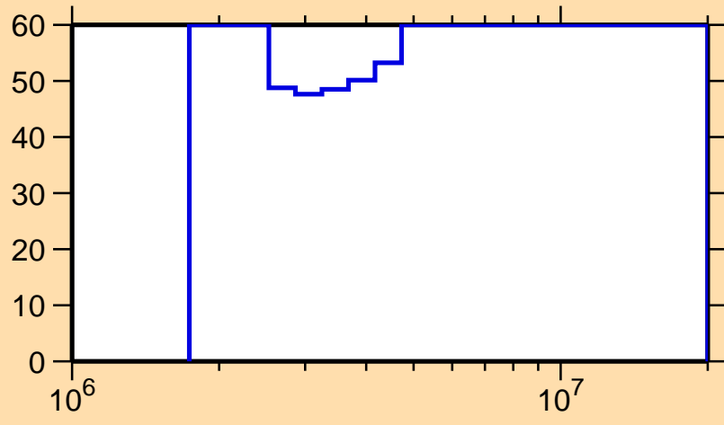
\Delta\sigma/\sigma vs. E for ^{173}\text{Er}(n,\gamma)
