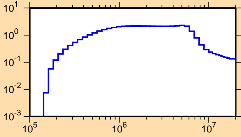
\sigma vs. E for ^{173}\text{Er}(n,n\text{cont.})
