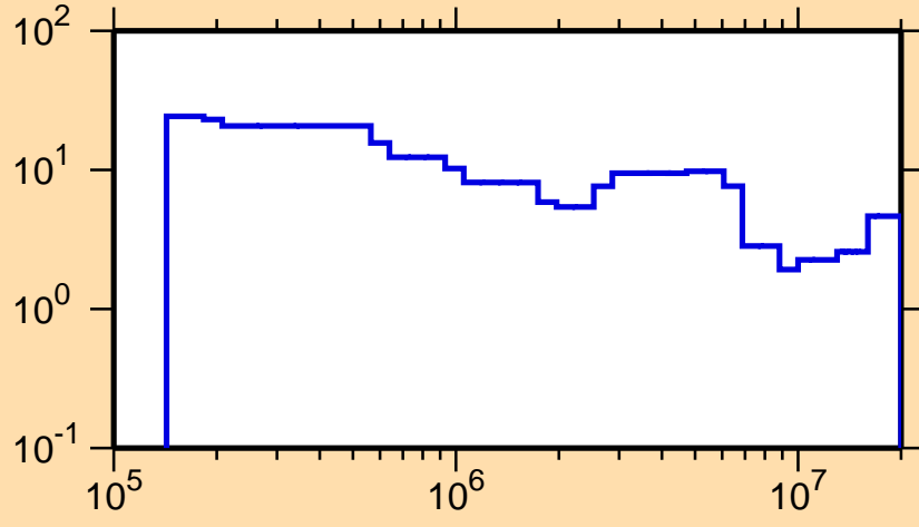
\Delta\sigma/\sigma vs. E for ^{173}\text{Er}(n, el.)
