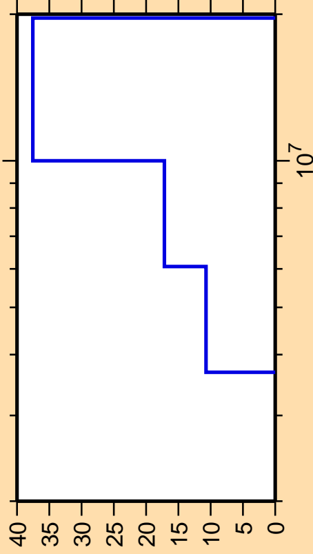
\Delta\sigma/\sigma vs. E for ^{173}\text{Er}(n,n\text{cont.})
