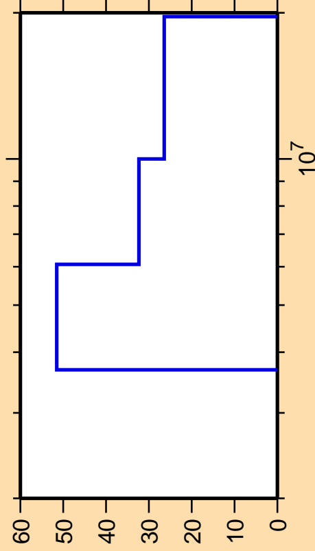
\Delta\sigma/\sigma vs. E for ^{173}\text{Er}(n,n_1)
