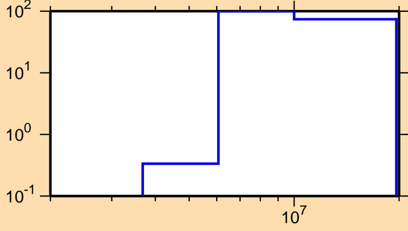
\Delta\sigma/\sigma vs. E for ^{173}\text{Er}(n,p)
