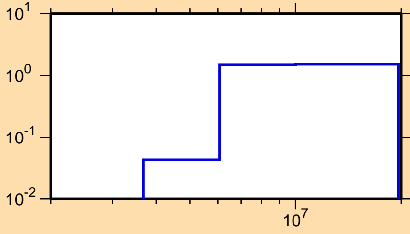
\sigma vs. E for ^{173}\text{Er}(n,2n)
