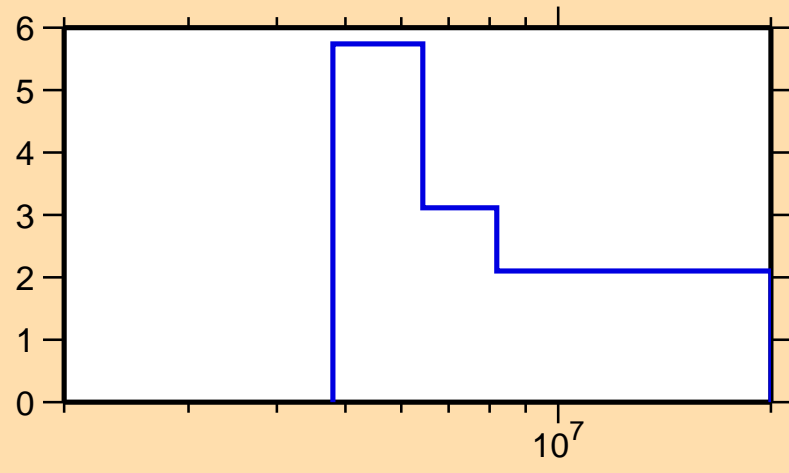
\Delta\sigma/\sigma vs. E for ^{173}\text{Er}(n,\text{tot.})
