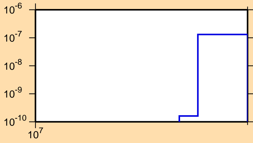
\sigma vs. E for ^{174}\text{Er}(n,nt)
