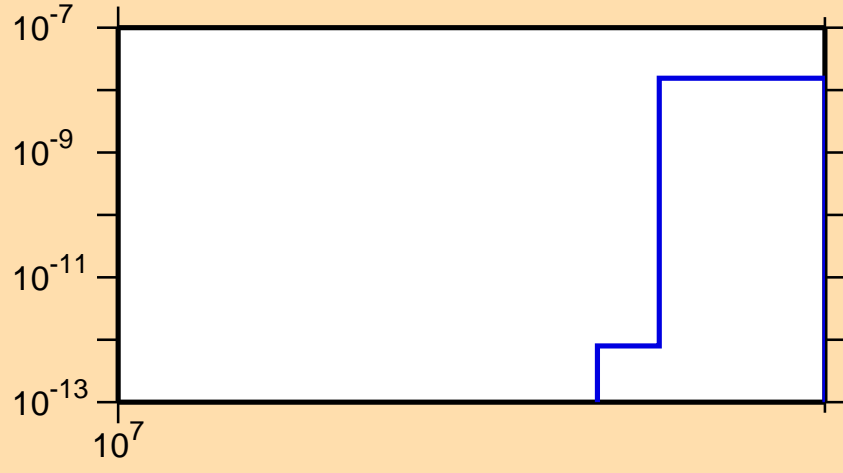
\sigma vs. E for ^{174}\text{Er}(n,\text{nd})
