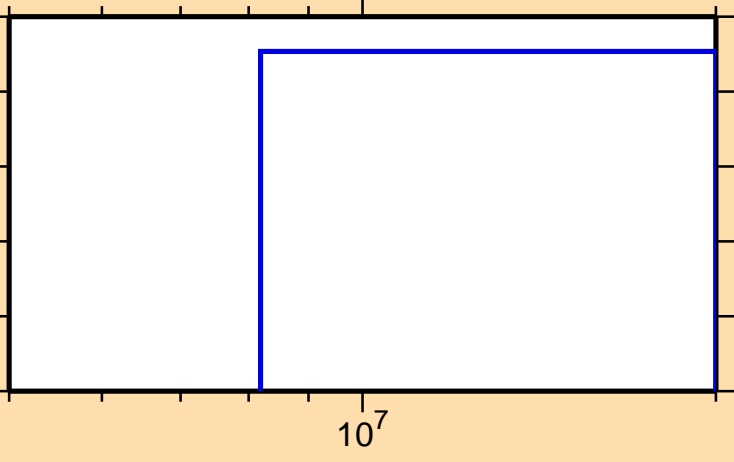
\sigma vs. E for ^{174}\text{Er}(n,np)
