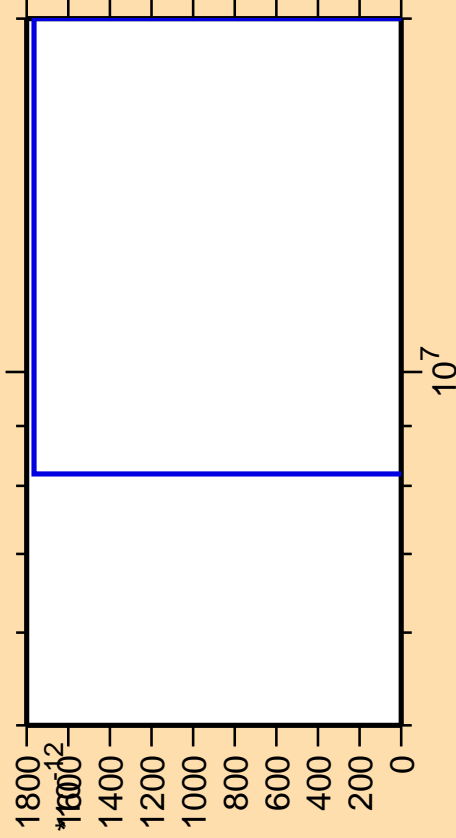
\Delta\sigma/\sigma vs. E for ^{174}\text{Er}(\text{mt } 11)
