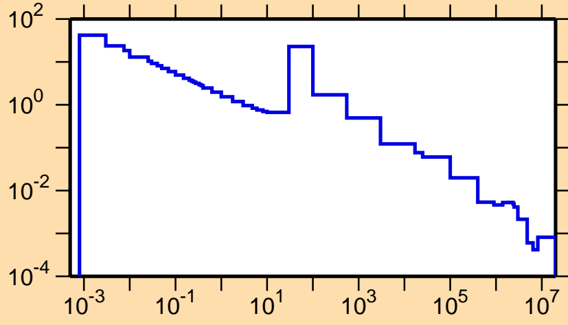
\sigma vs. E for ^{174}\text{Er}(n,\gamma)
