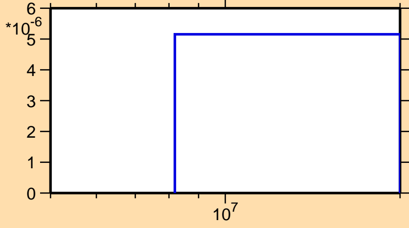
\sigma vs. E for ^{174}\text{Er}(n,t)
