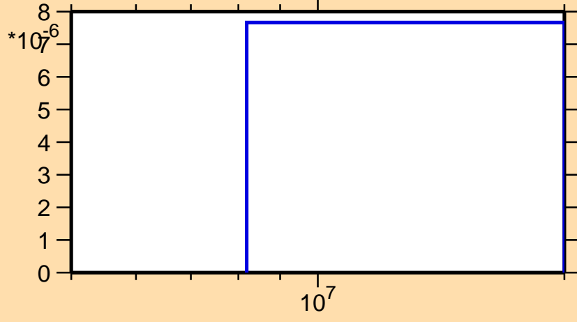
\sigma vs. E for ^{175}\text{Er}(n,t)
