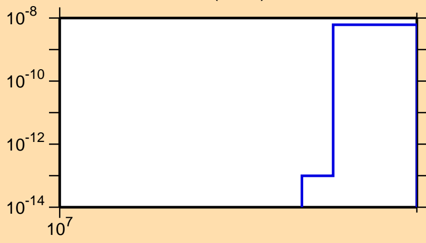
\sigma vs. E for ^{176}\text{Er}(n,\text{nd})
