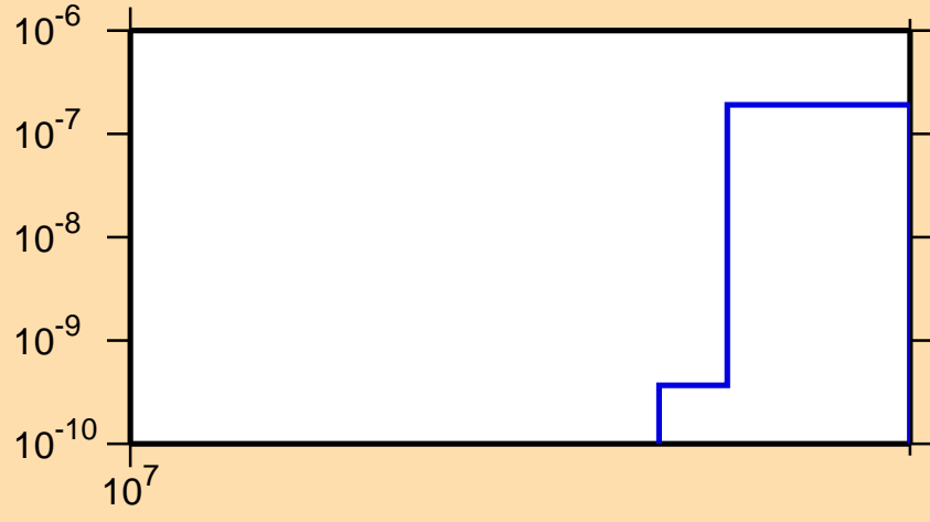
\sigma vs. E for ^{176}\text{Er}(n,nt)
