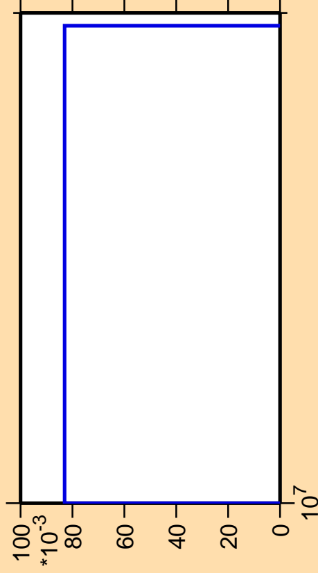
\Delta\sigma/\sigma vs. E for ^{176}\text{Er}(n,2np)
