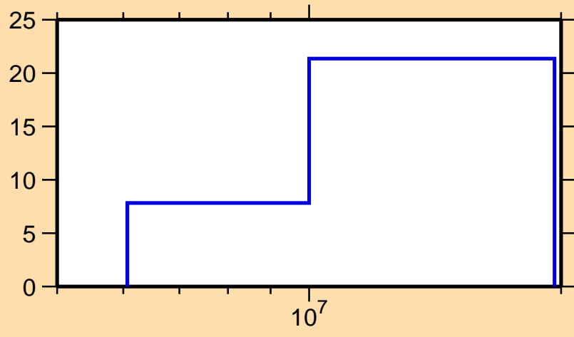
\Delta\sigma/\sigma vs. E for ^{176}\text{Er}(n,n\text{cont.})
