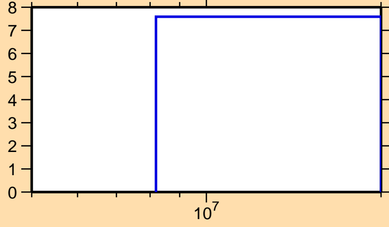
\Delta\sigma/\sigma vs. E for ^{176}\text{Er}(n,\text{el.})
