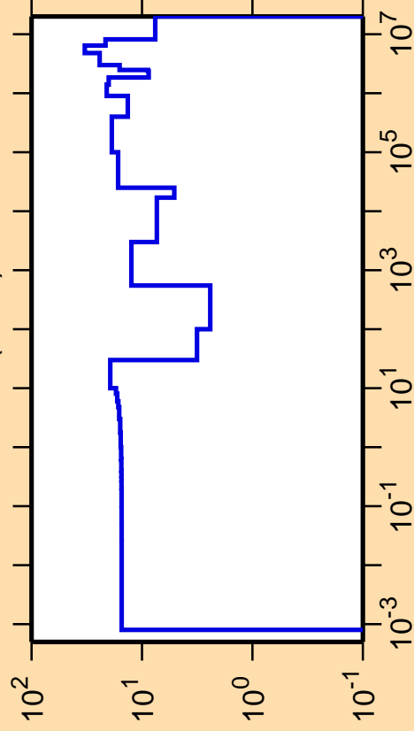
\Delta\sigma/\sigma vs. E for ^{176}\text{Er}(n,\text{el.})
