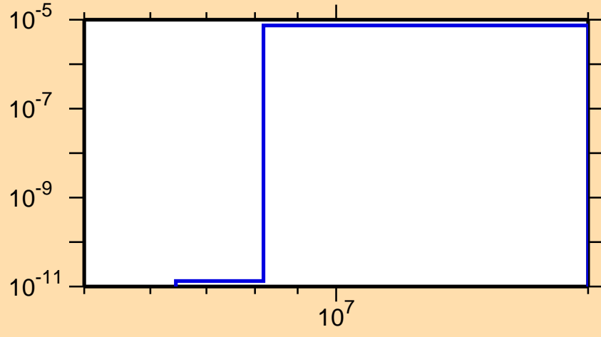
\sigma vs. E for ^{176}\text{Er}(n,\alpha)
