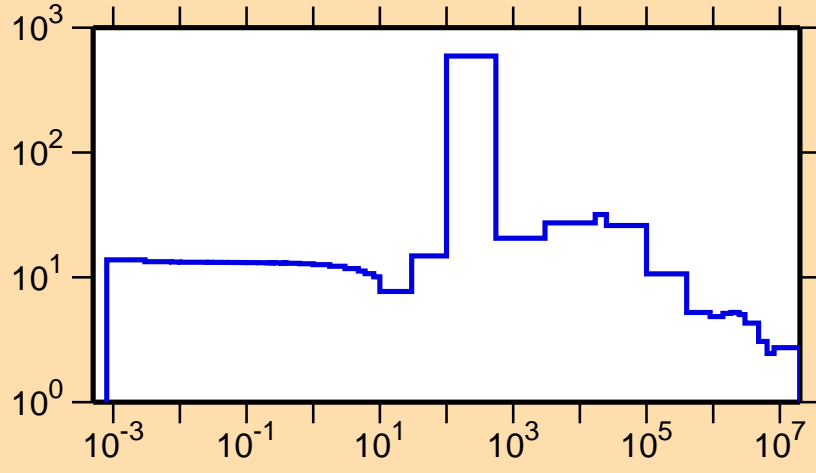
\sigma vs. E for ^{176}\text{Er}(n,\text{el.})
