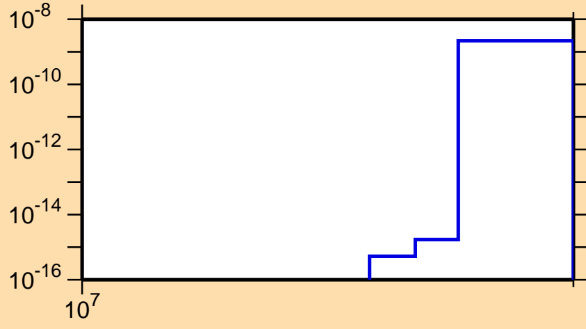
\sigma vs. E for ^{177}\text{Er}(n,2np)
