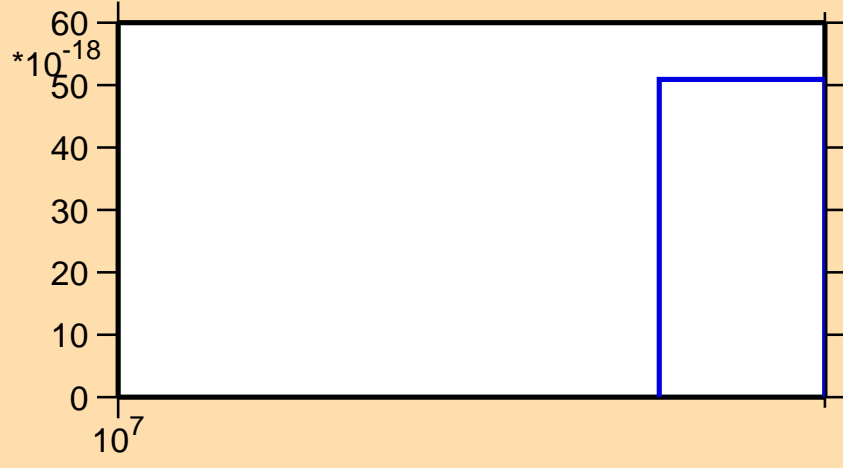
\sigma vs. E for ^{177}\text{Er}(\text{mt } 11)
