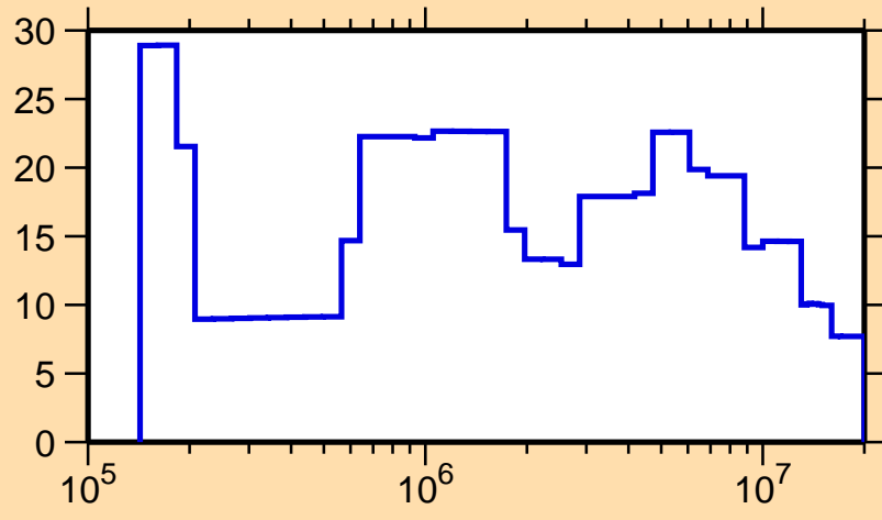
\Delta\sigma/\sigma vs. E for ^{177}\text{Er}(n, el.)
