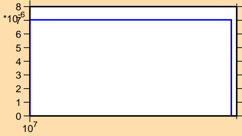
\sigma vs. E for ^{177}\text{Er}(n,d)
