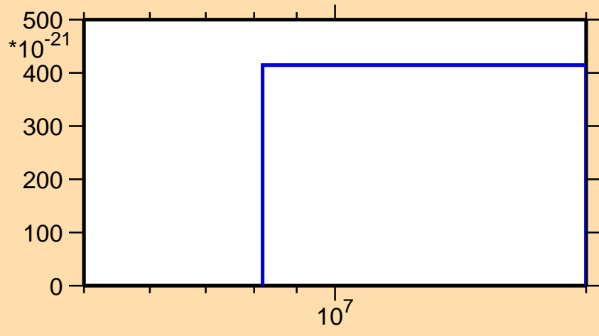
\sigma vs. E for ^{177}\text{Er}(\text{mt } 11)
