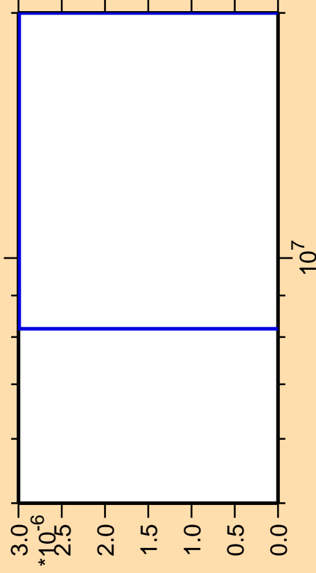
\Delta\sigma/\sigma vs. E for ^{177}\text{Er}(\text{mt } 11)
