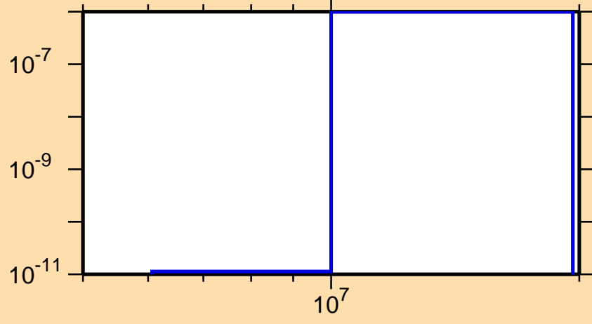
\sigma vs. E for ^{239}\text{Es}(n,\text{He3})
