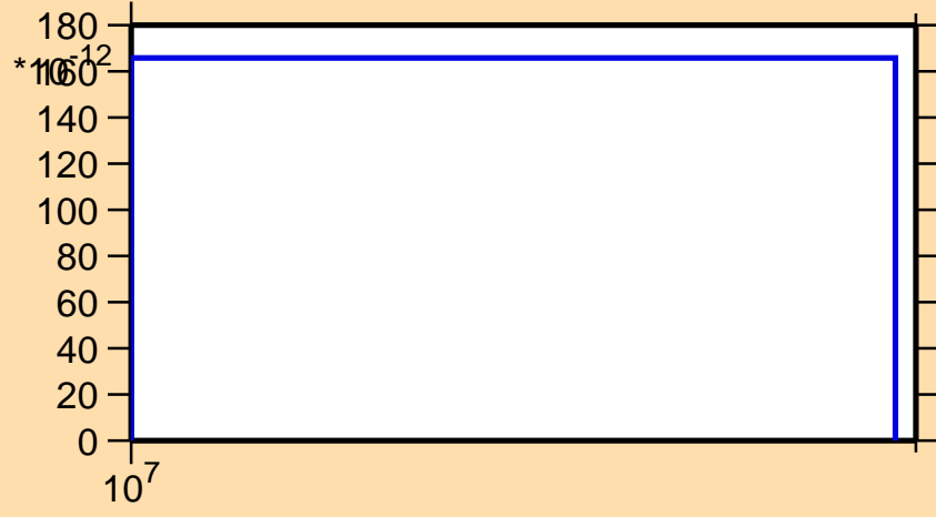
\sigma vs. E for ^{239}\text{Es} (mt 45)
