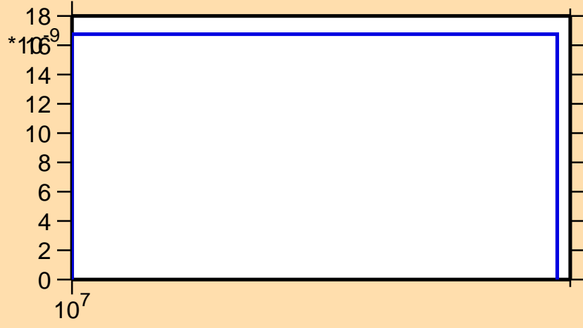
\sigma vs. E for ^{239}\text{Es}(n,pd)
