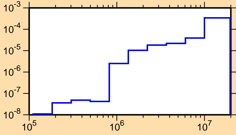
\sigma vs. E for ^{239}\text{Es}(n,n\alpha)
