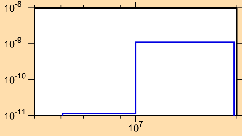
\sigma vs. E for ^{239}\text{Es}(n,p\alpha)
