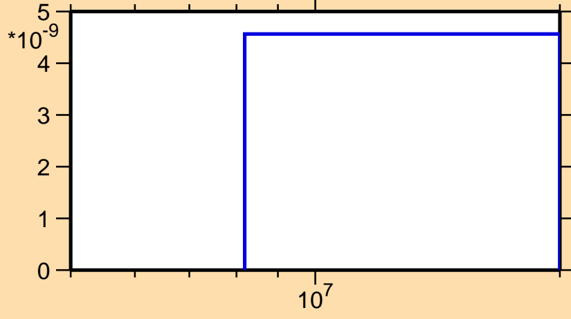
\sigma vs. E for ^{239}\text{Es}(\text{mt117})
