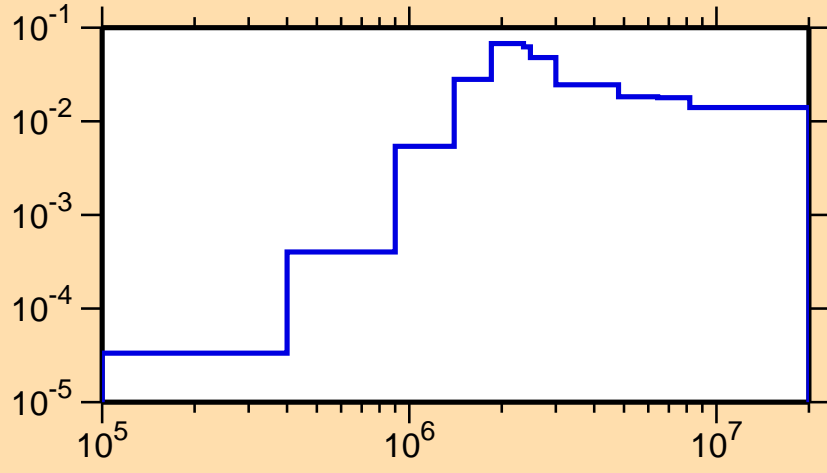
\sigma vs. E for ^{239}\text{Es}(n,n\text{cont.})
