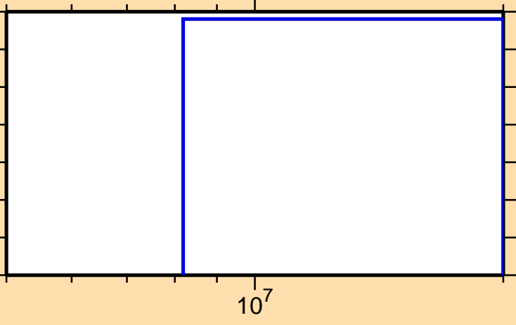
\sigma vs. E for ^{239}\text{Es}(n,pd)
