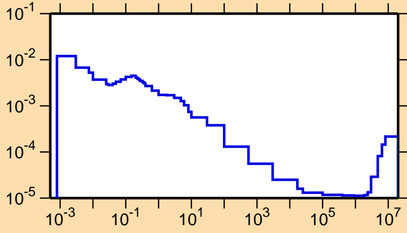
\sigma vs. E for ^{239}\text{Es}(n,p)
