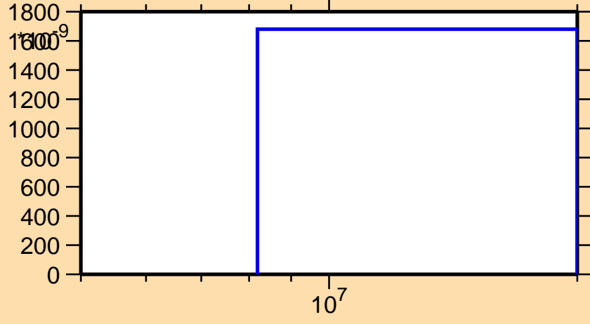
\sigma vs. E for ^{239}\text{Es}(n,2n\alpha)
