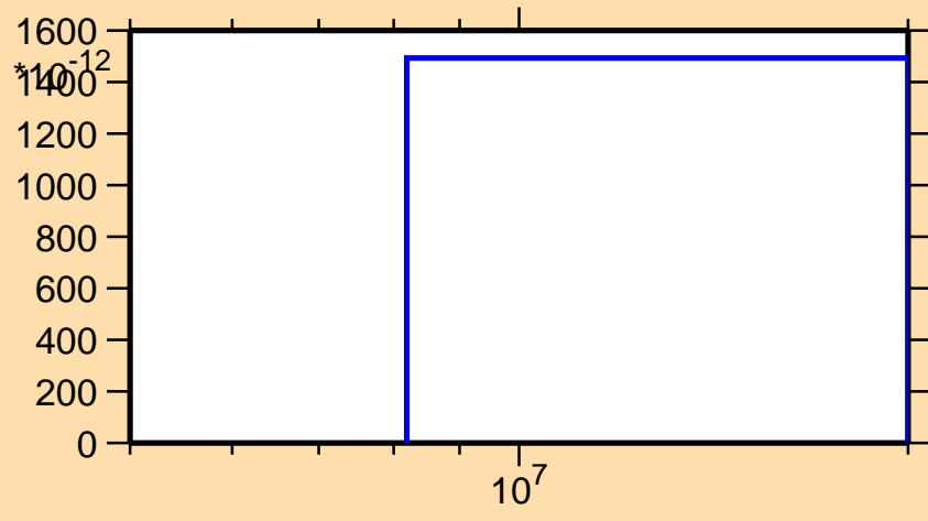
\sigma vs. E for ^{239}\text{Es}(n,nd)
