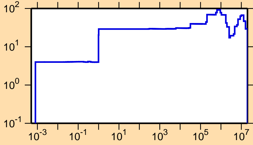
\Delta\sigma/\sigma vs. E for ^{240}\text{Es}(n,el.)
