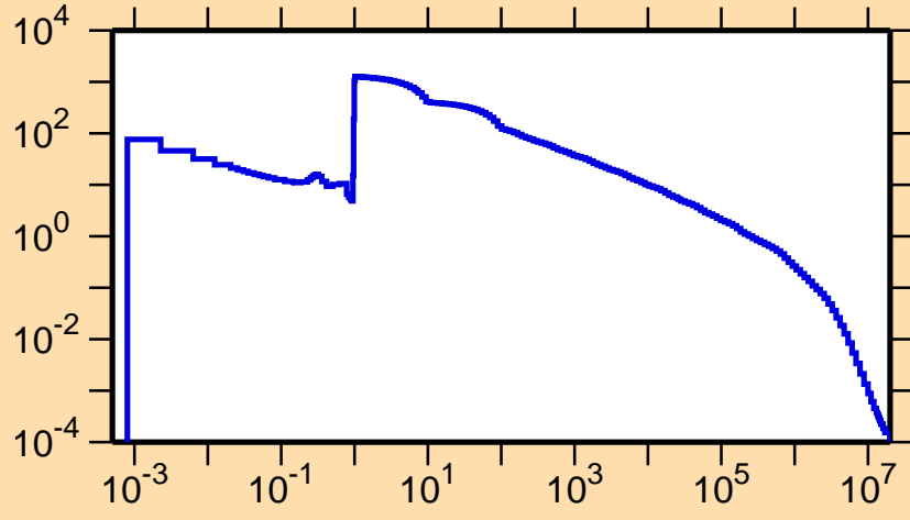
\sigma vs. E for ^{240}\text{Es}(n,\gamma)
