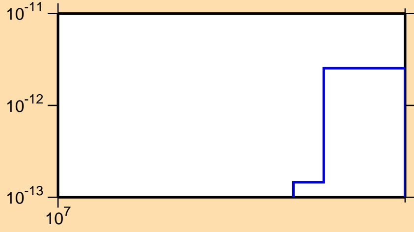
\sigma vs. E for ^{240}\text{Es}(n,nt)
