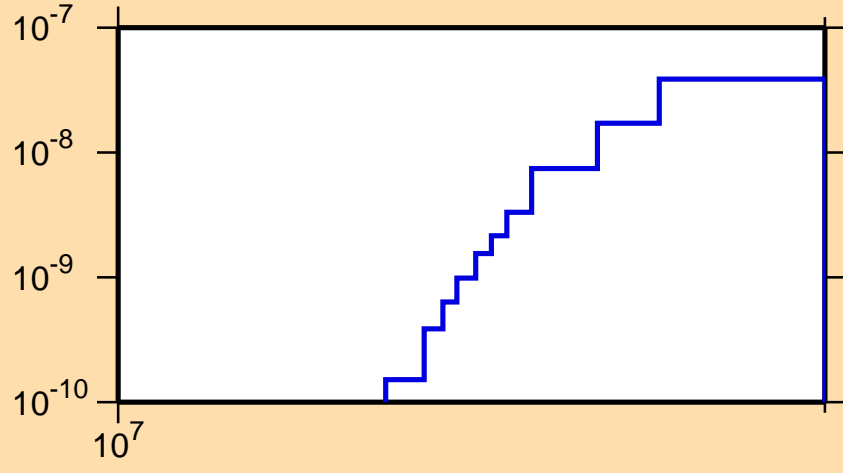
\sigma vs. E for ^{240}\text{Es}(n,2np)
