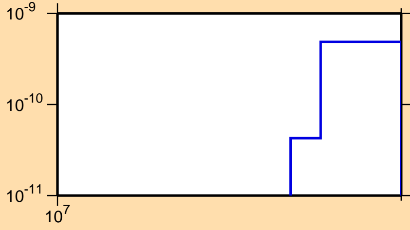
\sigma vs. E for ^{240}\text{Es}(n,3n\alpha)
