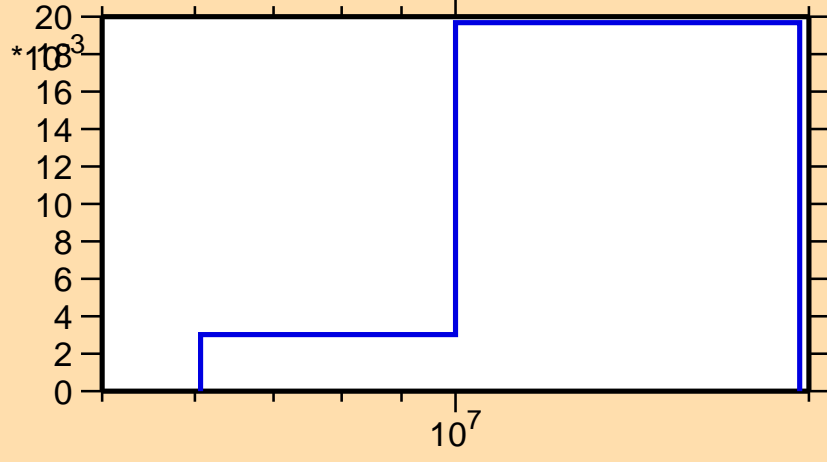
\sigma vs. E for ^{240}\text{Es}(n,2n)
