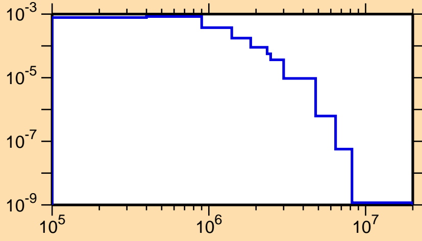
\sigma vs. E for ^{240}\text{Es}(n,n_1)
