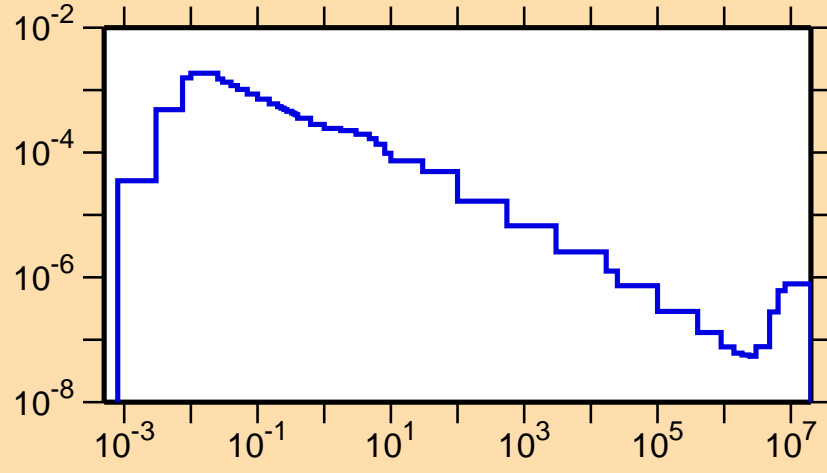
\sigma vs. E for ^{240}\text{Es}(n,\alpha)
