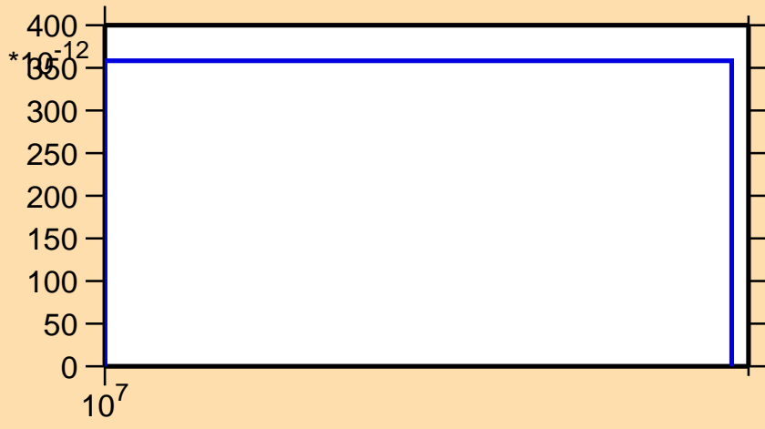
\sigma vs. E for ^{241}\text{Es}(n,\text{nd})
