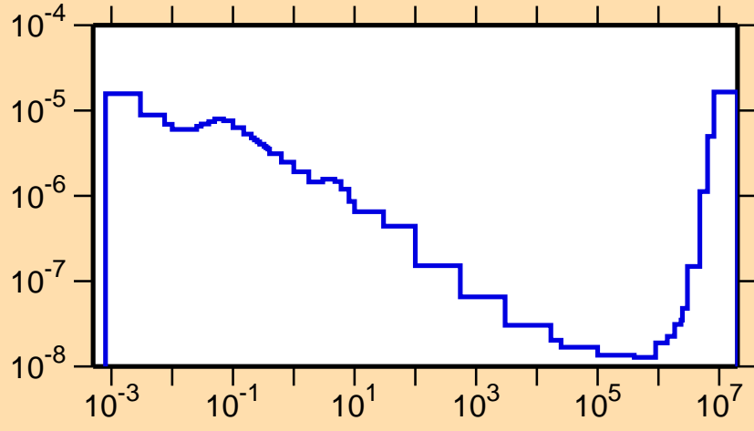
\sigma vs. E for ^{241}\text{Es}(n,\alpha)
