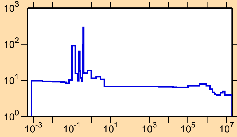
\sigma vs. E for ^{241}\text{Es}(n,el.)
