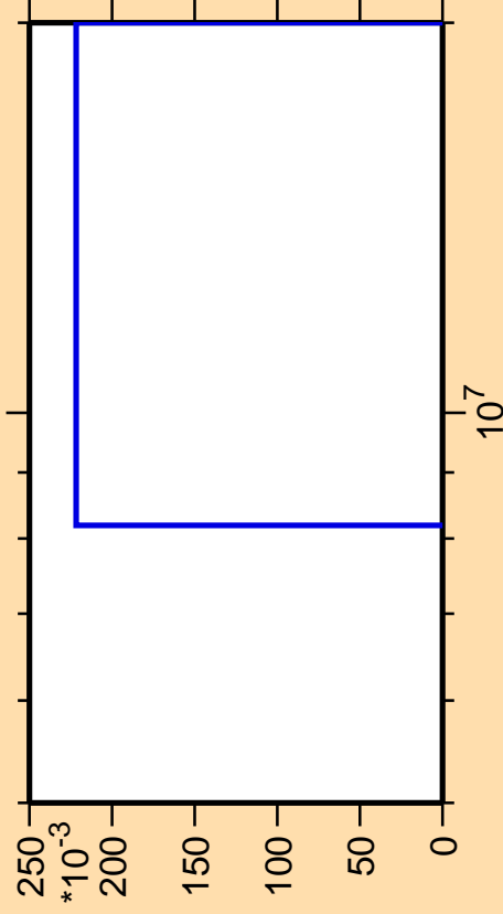
\Delta\sigma/\sigma vs. E for ^{241}\text{Es}(n,3n\alpha)
