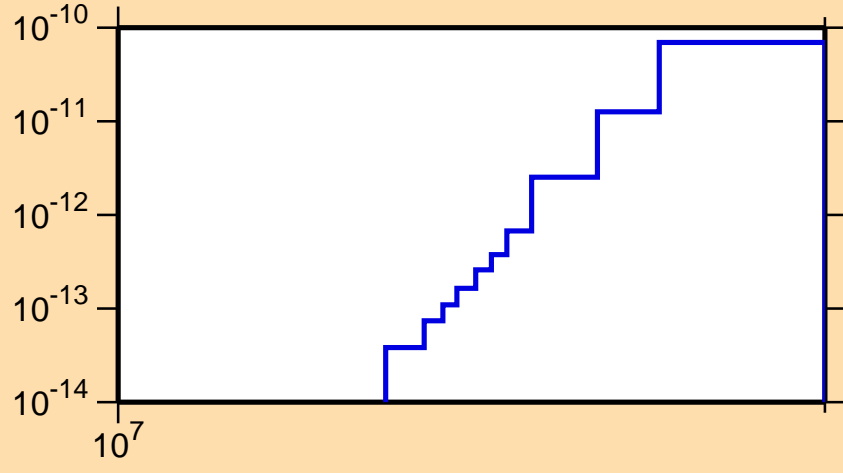
\sigma vs. E for ^{242}\text{Es}(\text{mt117})
