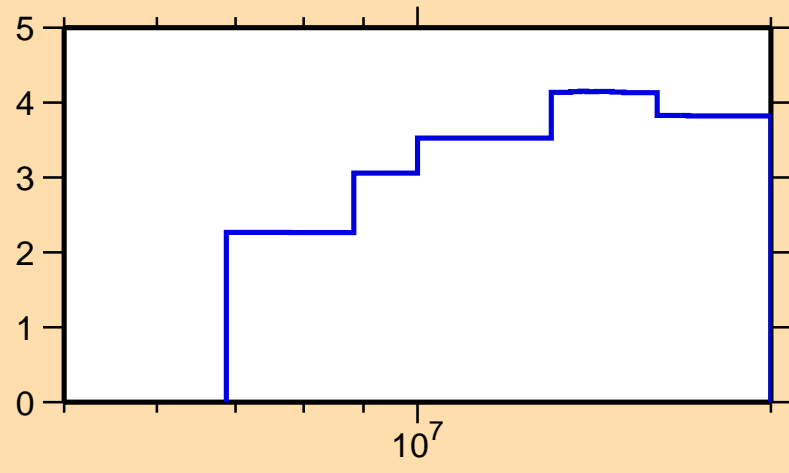
\Delta\sigma/\sigma vs. E for ^{242}\text{Es}(n,\text{nonel.})
