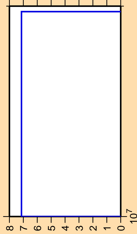
\Delta\sigma/\sigma vs. E for ^{242}\text{Es}(\text{mt117})
