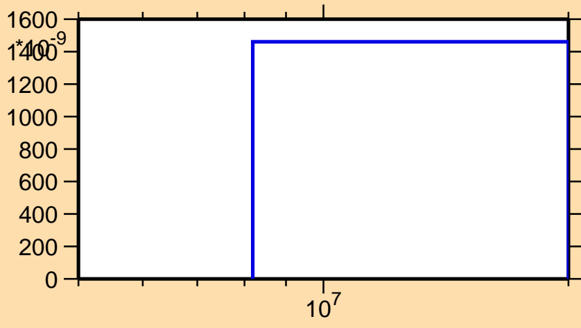
\sigma vs. E for ^{242}\text{Es}(n,2np)
