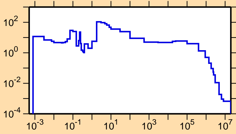
\sigma vs. E for ^{242}\text{Es}(n,\gamma)
