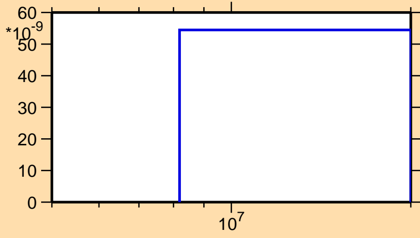
\sigma vs. E for ^{242}\text{Es}(n,nd)
