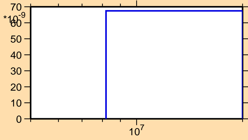
\sigma vs. E for ^{242}\text{Es}(n,\text{He3})
