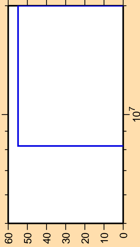
\Delta\sigma/\sigma vs. E for ^{242}\text{Es} (mt 34)
