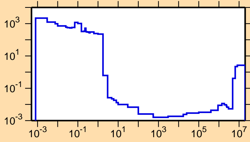
\sigma vs. E for ^{242}\text{Es}(n,f)
