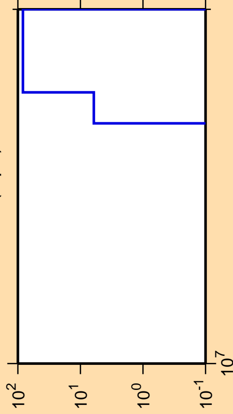
\Delta\sigma/\sigma vs. E for ^{243}\text{Es}(n,pd)
