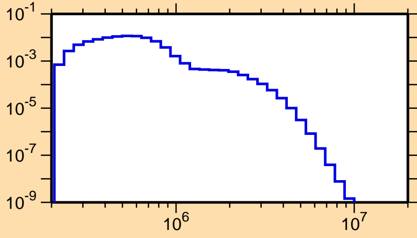
\sigma vs. E for ^{243}\text{Es}(n,n_1)
