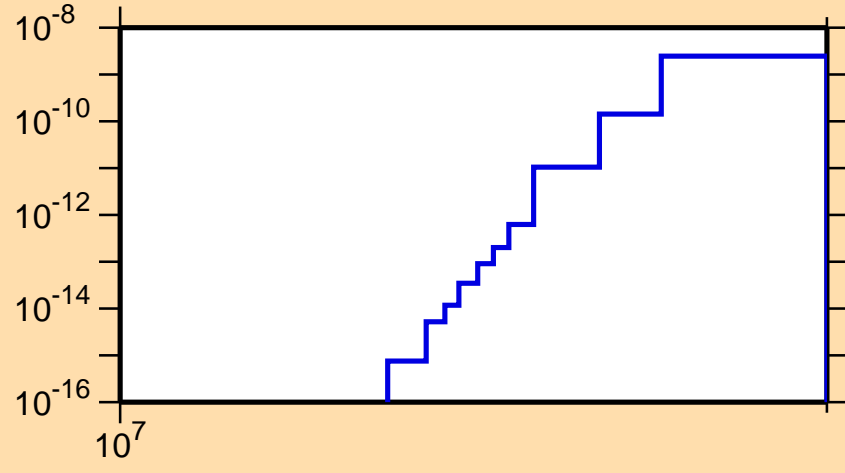
\sigma vs. E for ^{243}\text{Es}(n,nt)
