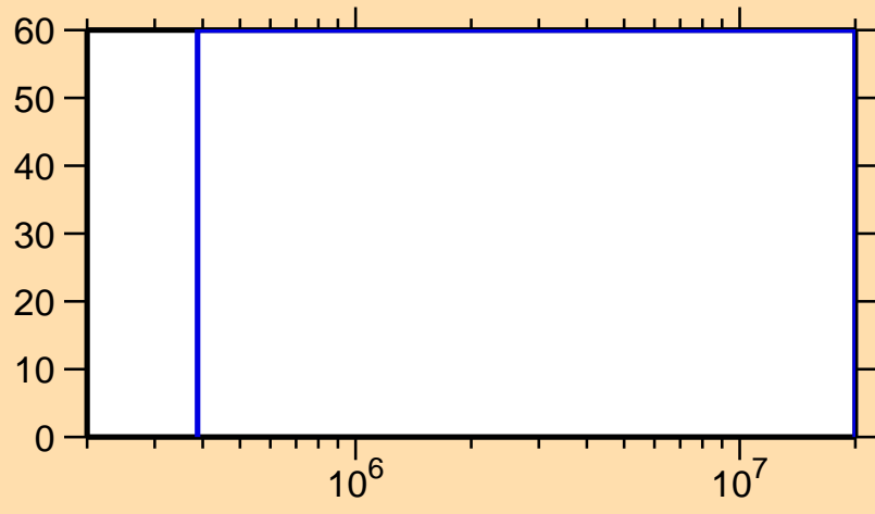
\Delta\sigma/\sigma vs. E for ^{243}\text{Es}(n,n\text{cont.})
