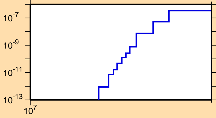
\sigma vs. E for ^{243}\text{Es}(n,2np)
