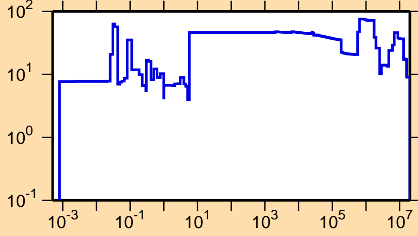
\Delta\sigma/\sigma vs. E for ^{243}\text{Es}(n,el.)
