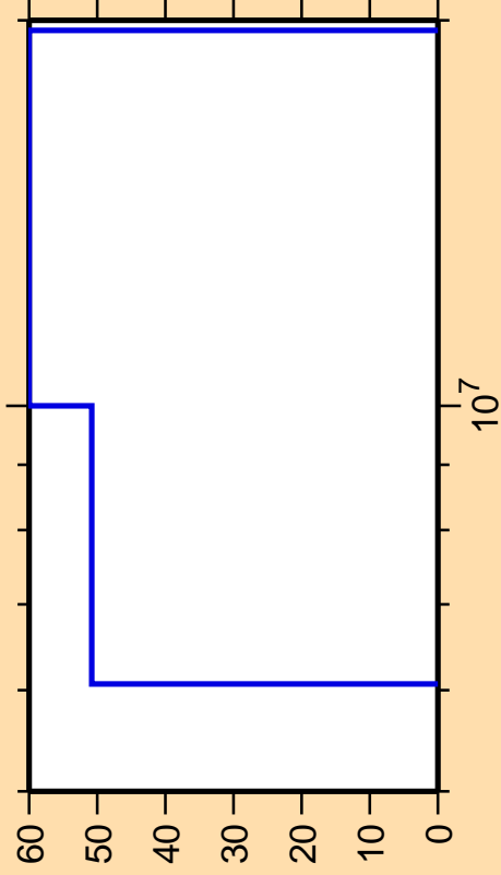
\Delta\sigma/\sigma vs. E for ^{243}\text{Es}(n,p\alpha)
