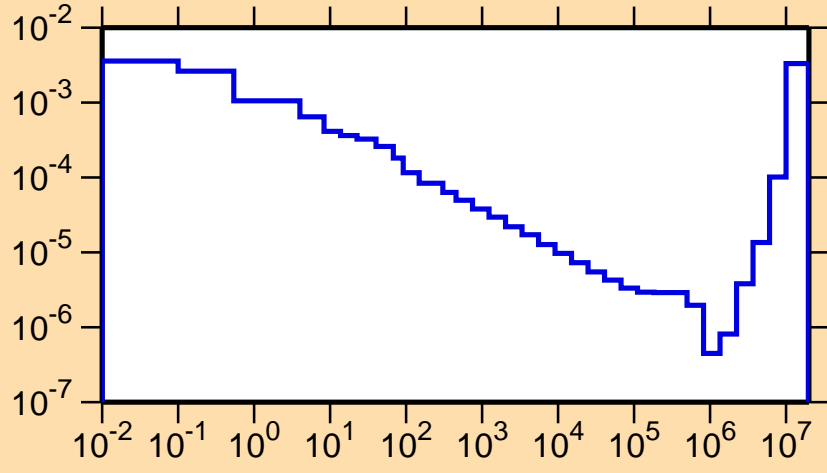
\sigma vs. E for ^{243}\text{Es}(n,\alpha)
