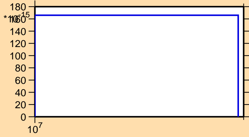
\sigma vs. E for ^{243}\text{Es}(n,pd)
