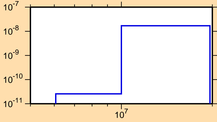
\sigma vs. E for ^{243}\text{Es}(n,p\alpha)
