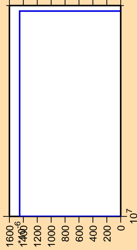
\Delta\sigma/\sigma vs. E for ^{243}\text{Es}(n,3n\alpha)
