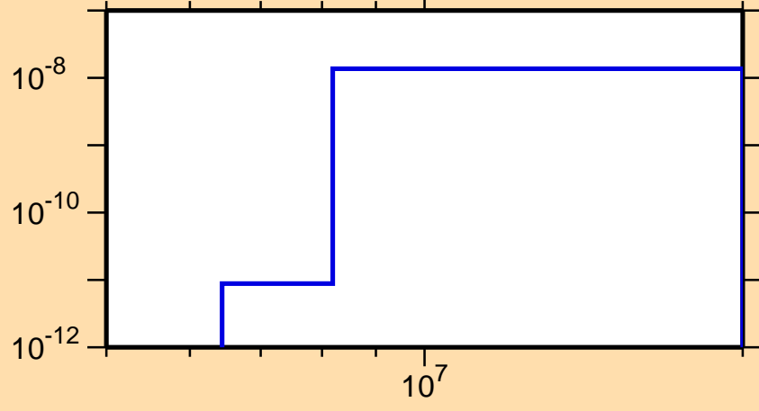
\sigma vs. E for ^{243}\text{Es}(n,p\alpha)
