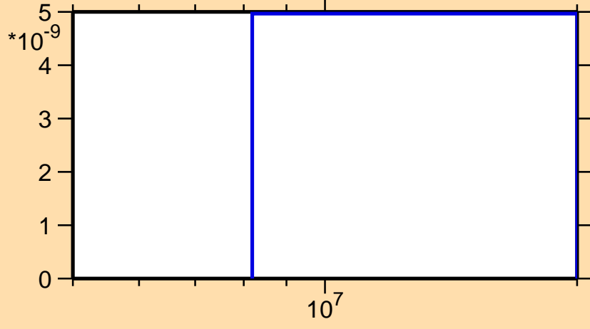
\sigma vs. E for ^{243}\text{Es}(n,nd)
