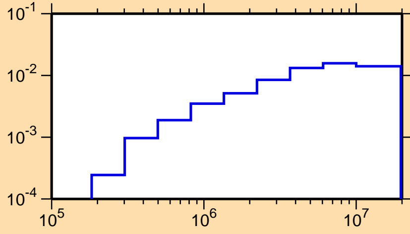
\sigma vs. E for ^{244}\text{Es}(n,n_2)
