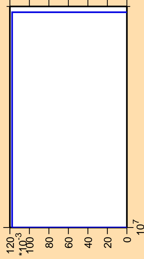
\Delta\sigma/\sigma vs. E for ^{244}\text{Es}(n,3n\alpha)
