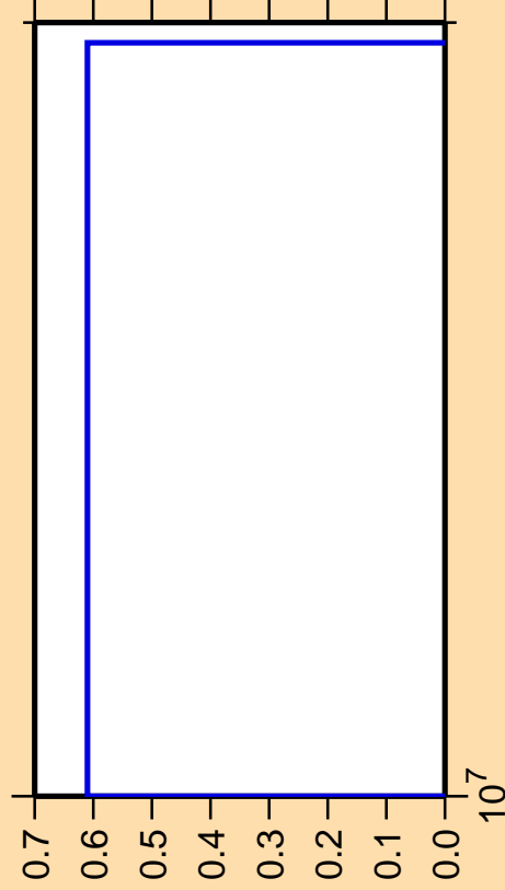
\Delta\sigma/\sigma vs. E for ^{244}\text{Es}(n,pd)
