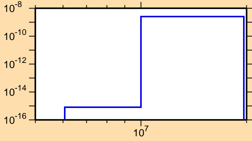
\sigma vs. E for ^{244}\text{Es}(n,\text{He3})
