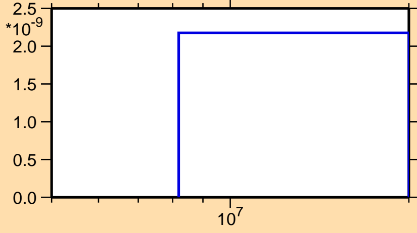
\sigma vs. E for ^{244}\text{Es}(n,p\alpha)
