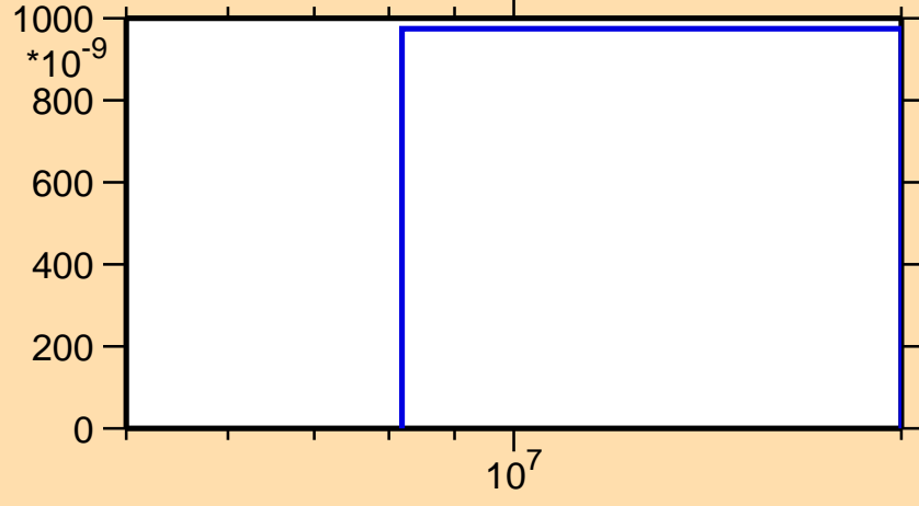
\sigma vs. E for ^{244}\text{Es}(n,nd)
