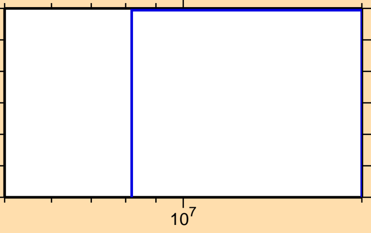
\sigma vs. E for ^{244}\text{Es}(n,2np)
